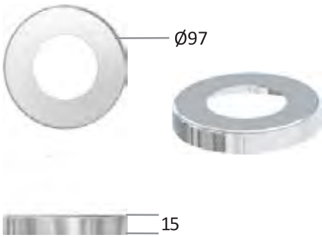
FLANGED
